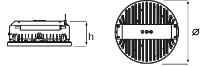
IP66 Lens
