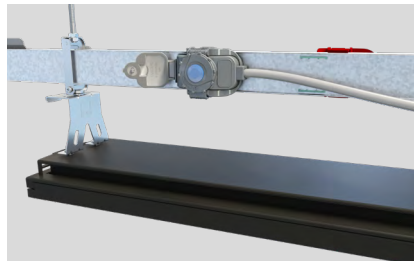
BUSBAR HANGER APPARATUS
